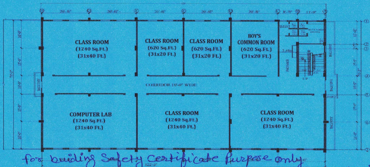
SECOND FLOOR
