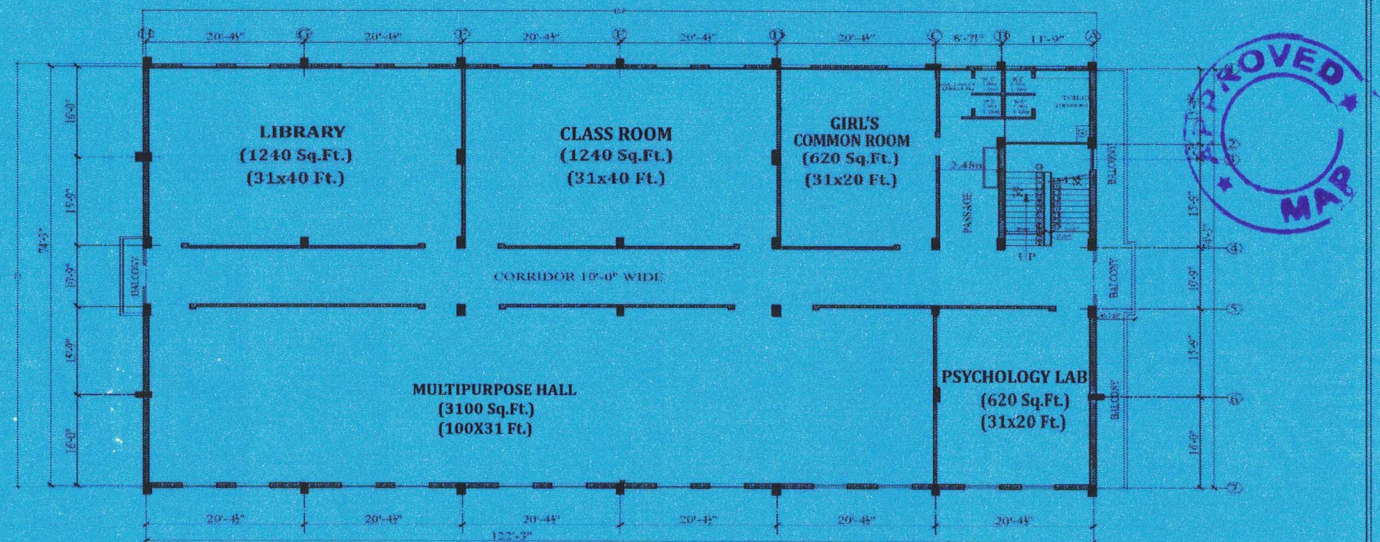
SECOND FLOOR
